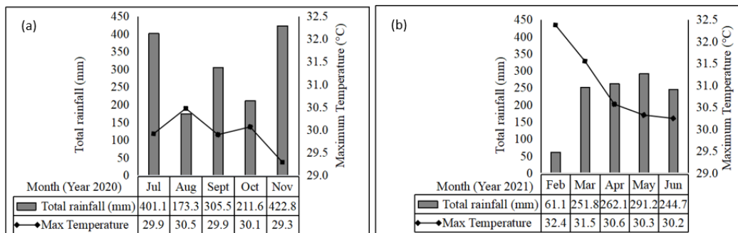
Fig. 1. Total rainfall and maximum temperature pattern during (a) Season 1 (July-November 2020) and (b) Season 2 (February-June 2021)
